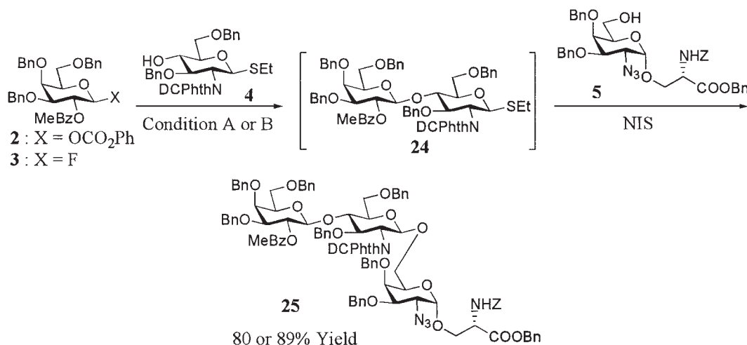
Scheme 9. Condition A: 2 (1.8 mol. amt.), 4 (1.0 mol. amt.), \text{TrB}(\text{C}_6\text{F}_5)_4 (0.30 mol. amt.), MS 5A, BTF, -15^\circ\text{C} , 5 h, then 5 (5.0 mol. amt.), NIS (2.0 mol. amt.), BTF- \text{CH}_2\text{Cl}_2 , -30^\circ\text{C} , 2 h, 80% (based on 4 ). Condition B: 3 (1.2 mol. amt.), 4 (1.0 mol. amt.), \text{TfOH} (0.20 mol. amt.), MS 5A, \text{CH}_2\text{Cl}_2 , -20^\circ\text{C} , 1 h, then 5 (1.5 mol. amt.), NIS (2.0 mol. amt.), \text{CH}_2\text{Cl}_2 , -20^\circ\text{C} , 1 h, 89% (based on 4 ).
